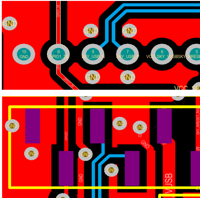
Figure 3: USB Signal Breakouts
