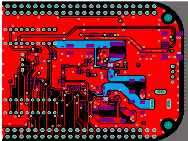
Figure 2: Low Impedance Power Path
