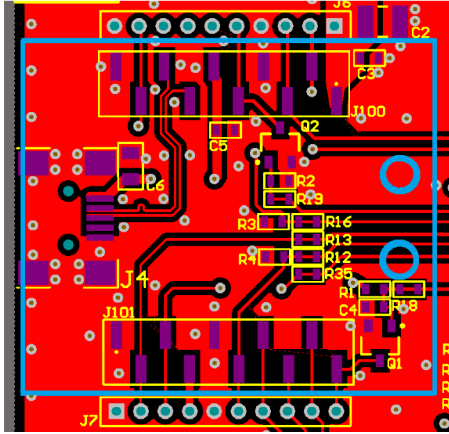
Figure 5: Silkscreen Markers
