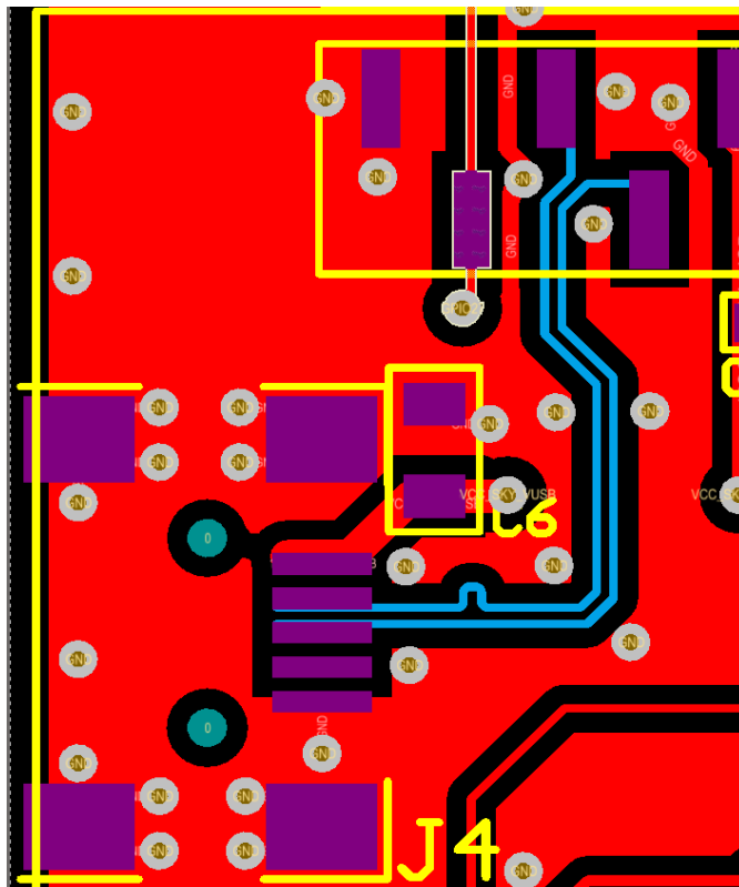
Figure 4: USB Routing
