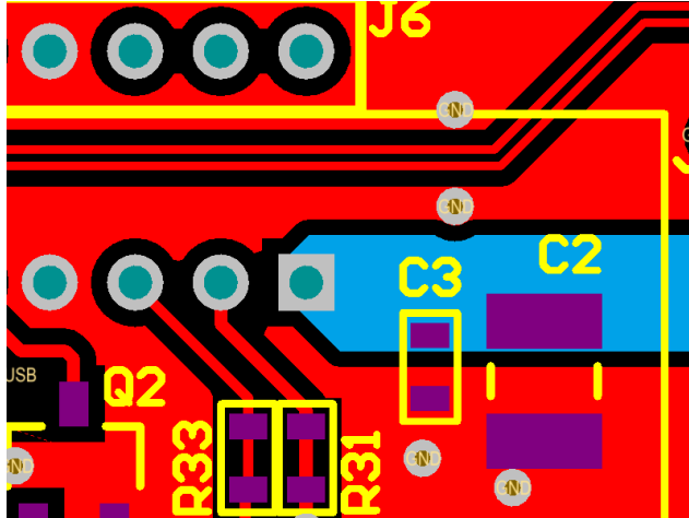
Figure 1: Decoupling Capacitor Placement
